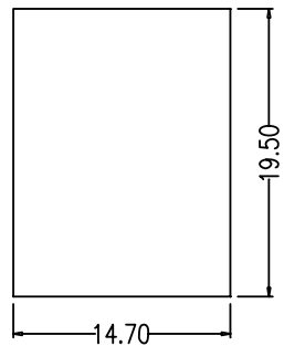
Suggested Panel Cutout
